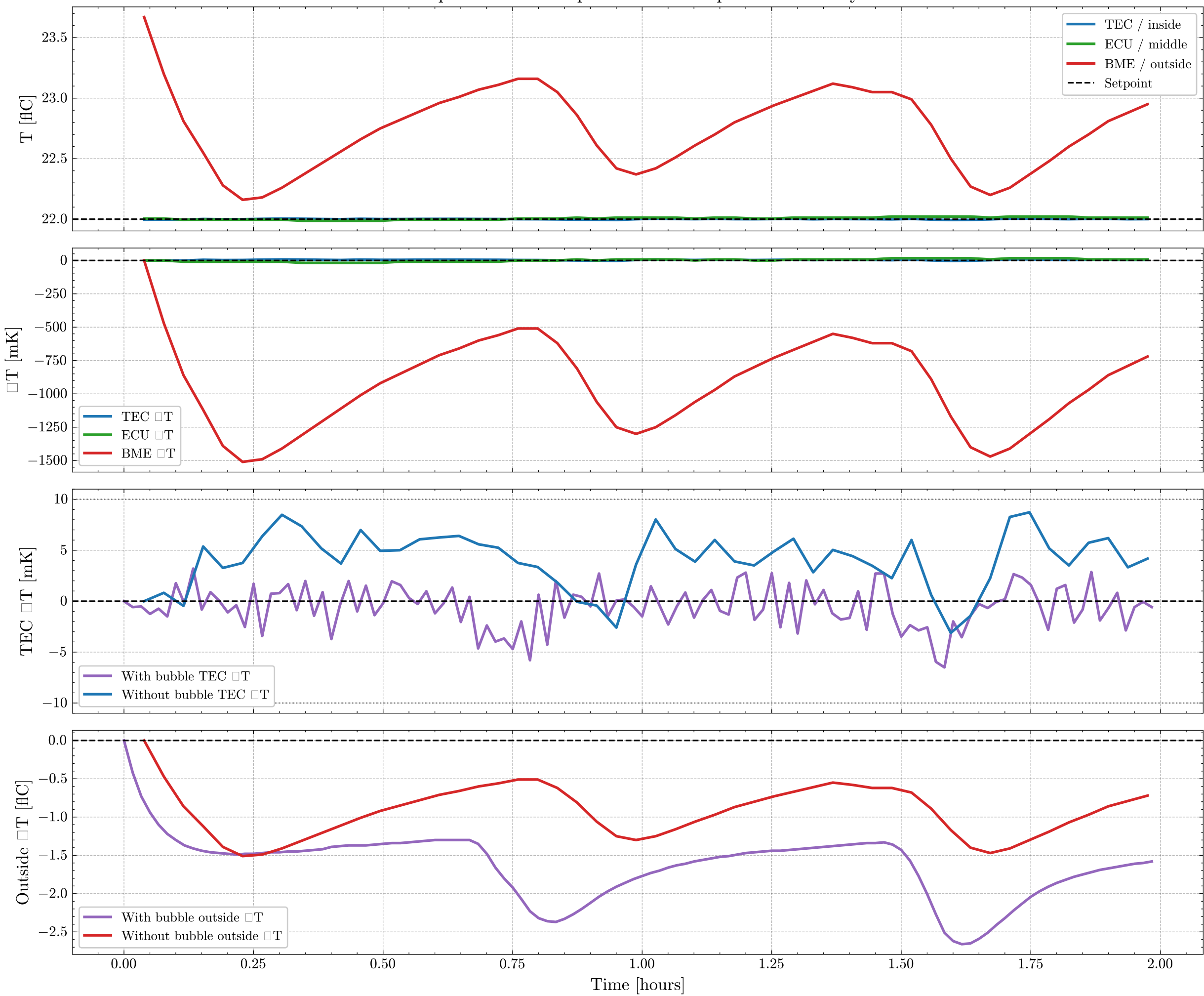
Experiment Warmup vs Bubble Temperature Stability
